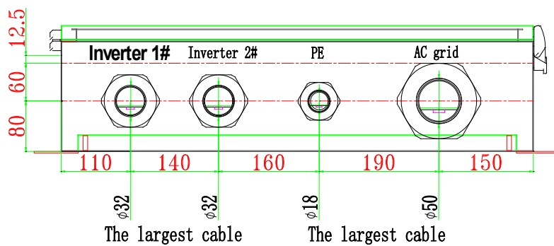
Bottom sketch
